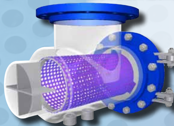
Suction Diffusers (FF Series)
